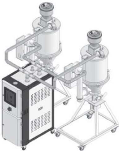
一对二成型机安装例图 Example of one to two installation diagram
